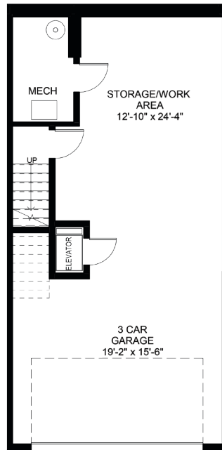
ENTRY LEVEL
