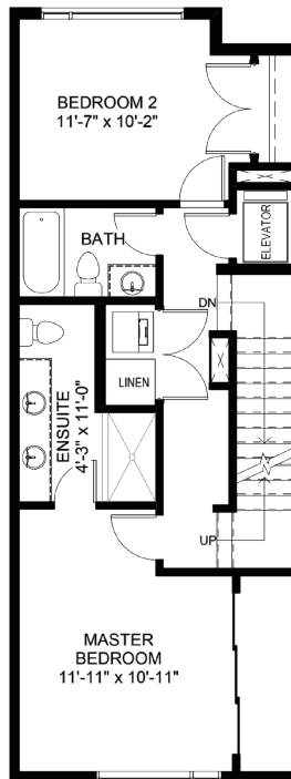
UPPER LEVEL
