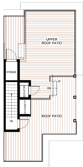
ROOF LEVEL
