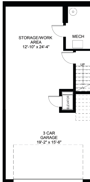
ENTRY LEVEL
