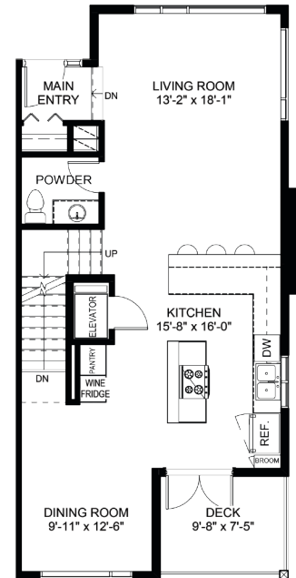
MAIN LEVEL
